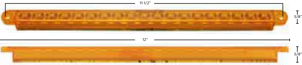
12 LED 12" Ultra Slim Turn Signal Light Bar Mounting holes approximately 11 1/2" apart
