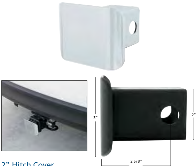
2" Hitch Cover
