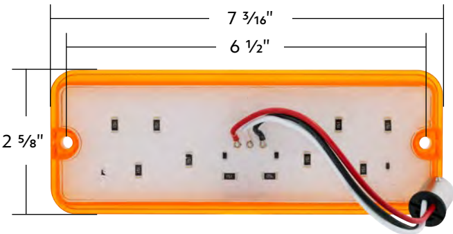
UP Item #111096 Amber LED / Clear Lens
