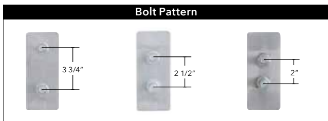
Bolt Pattern
