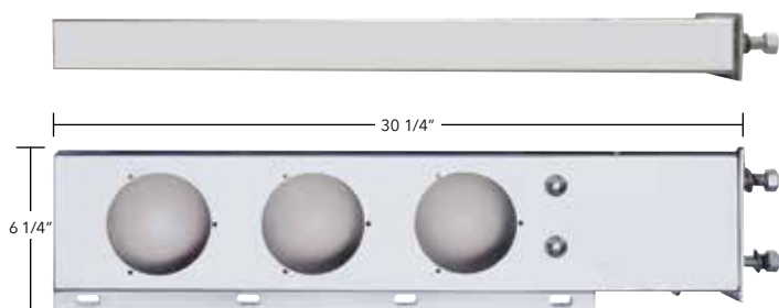
Bolt Pattern
