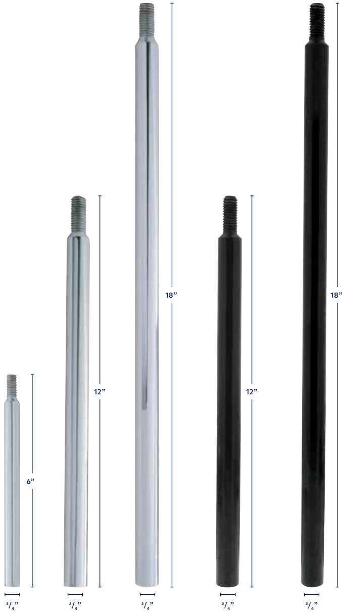
Chrome Shifter Shaft Extension • Thread on (1/2" - 13 UNC thread), thread 1" long, 3/4" diameter • For offroad use only
