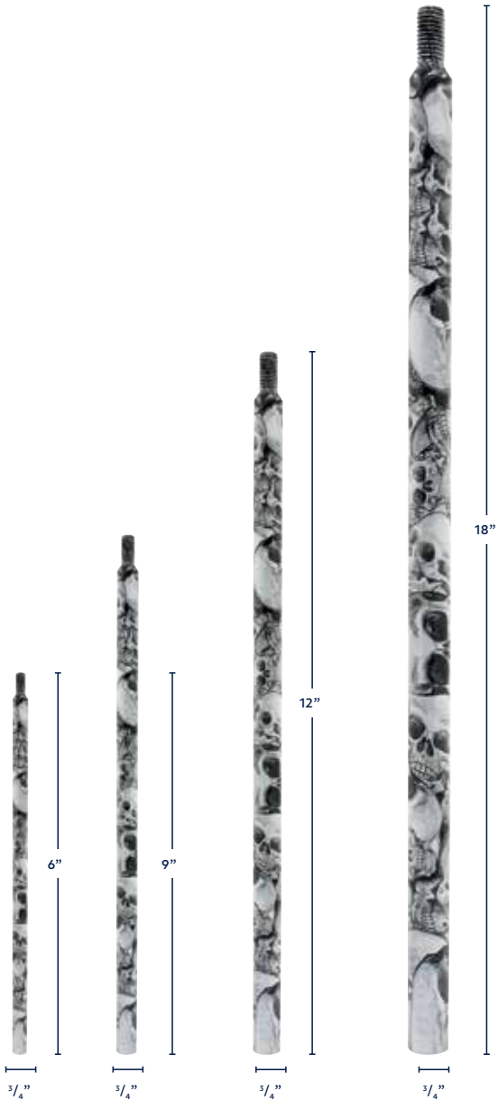
Skull Pattern Wrapped Shifter Shaft Extension • Thread on (1/2" - 13 UNC thread), thread 1" long, 3/4" diameter, fits up item #21740 • For offroad use only
