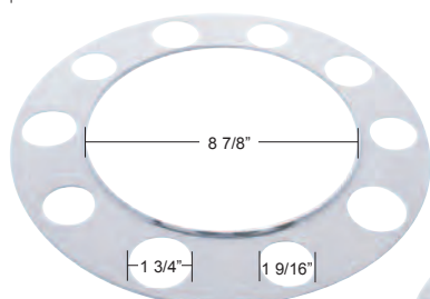
21214 Stud Piloted / Steel Wheel
