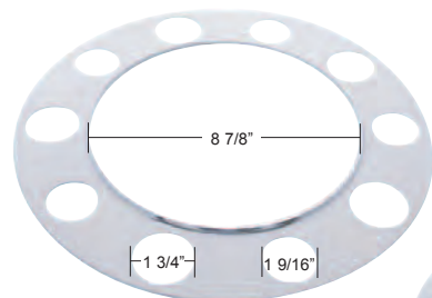
10214 Stud Piloted / Steel Wheel
