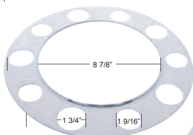
10214 Stud Piloted / Steel Wheel
