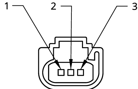
Side Marker/Repeater Plug
